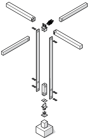
Beam construction
